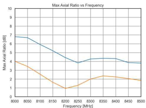
Figure 7-11: X-Band max axial vs frequency.
