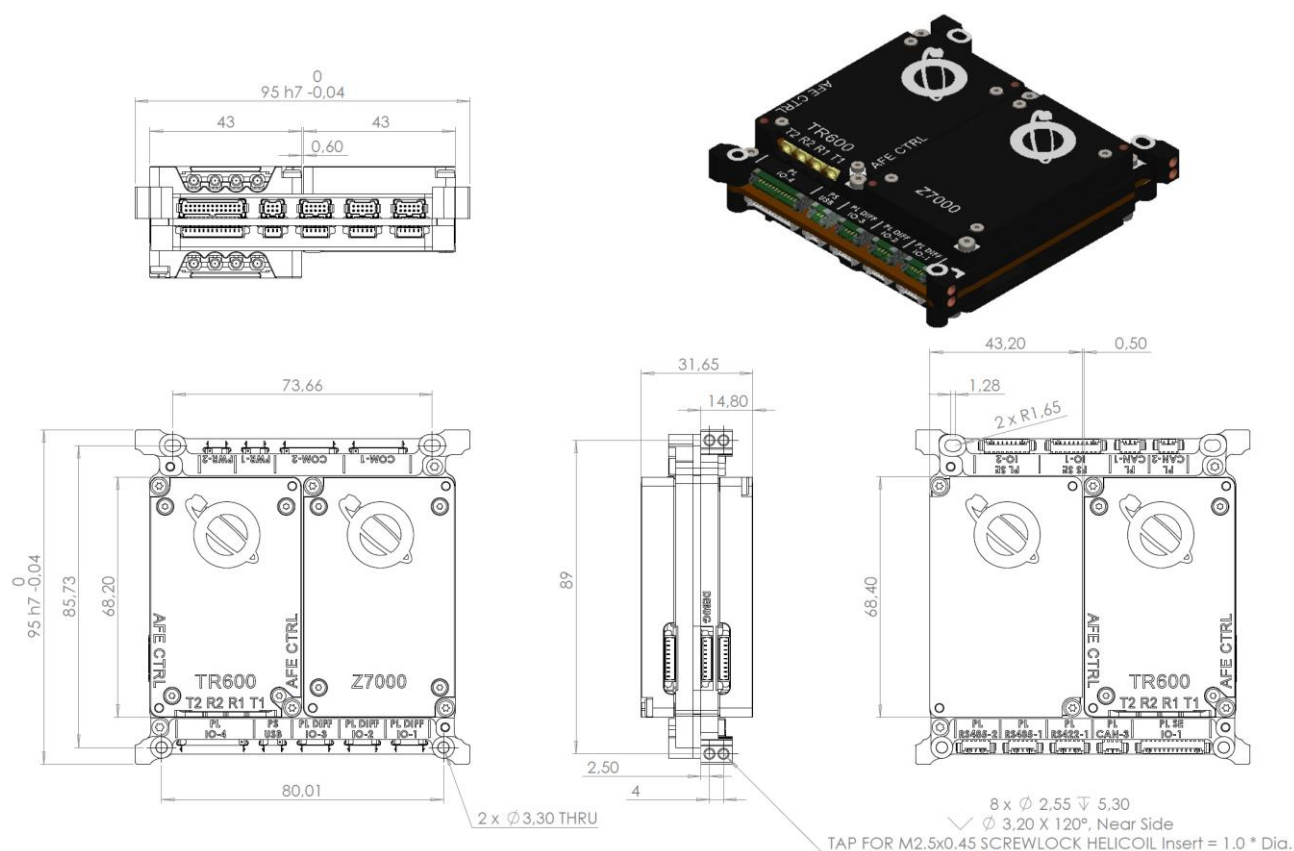
Figure 10-4: SDR MK3 – NanoCom Link SX.
