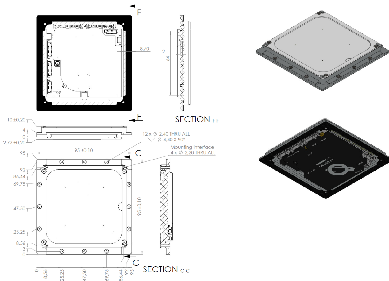
Figure 10-8: ANT8250 Backplate Y side.
