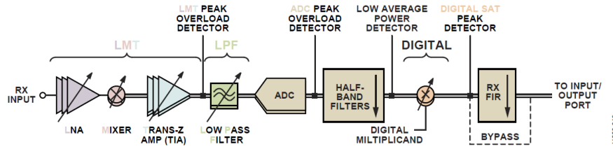
Figure 10.4.10.11. TR600 RX Gain stage Block Diagram
