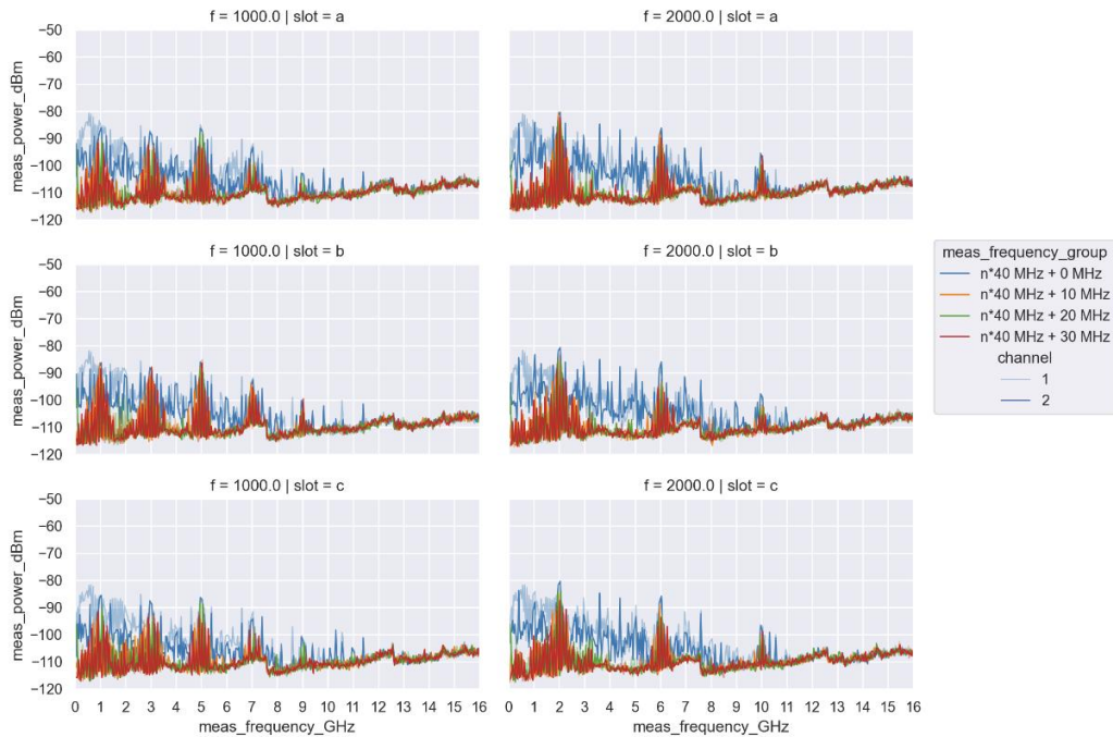
Figure 10.4.10.7. TX reference clock spurious level
