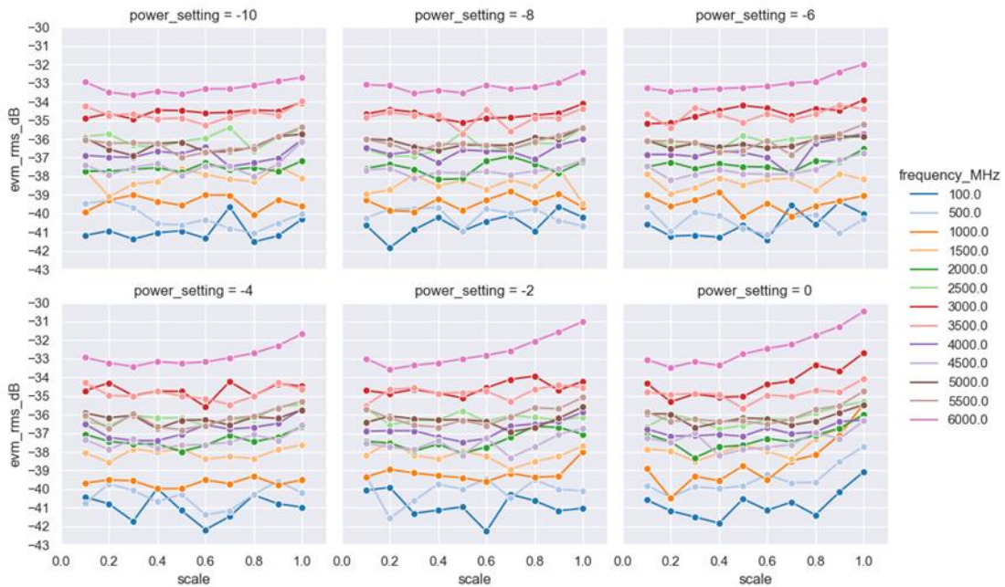
Figure 10.4.10.10. Typical EVM vs. power_setting vs. scale_setting
