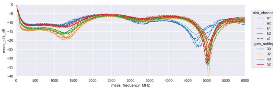
Figure 10.4.10.21. Typical S11 [dB]
