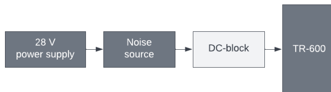
Figure 10.4.10.15: RX noise measurement
