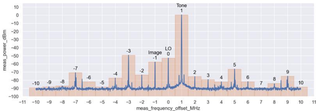
Figure 10.4.10.8. TX spurious near carrier. TX scale 0.7
