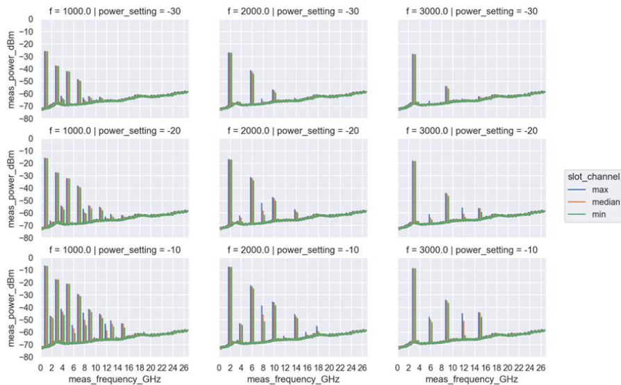
Figure 10.4.10.5: TX wideband emission
