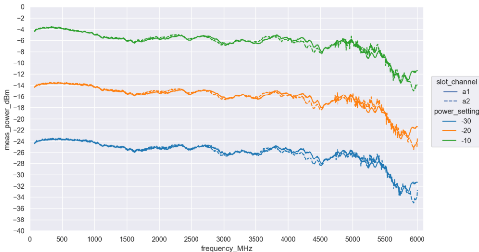
Figure 10.4.10.2. TX power vs. frequency and power_setting.
