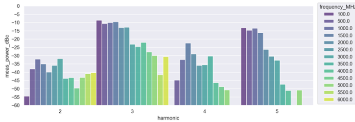
Figure 10.4.10.4. TX harmonics expressed as a level relative to the fundamental (dBc).
