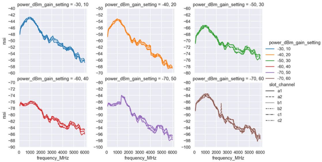
Figure 10.4.10.12. Typical RSSI report vs. power input and RX gain settings.
