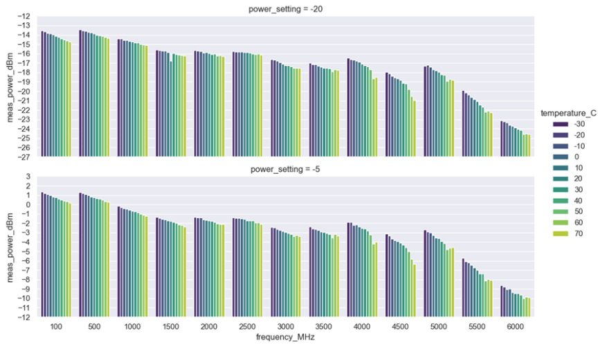
Figure 10.4.10.3. TX power vs. temperature.
