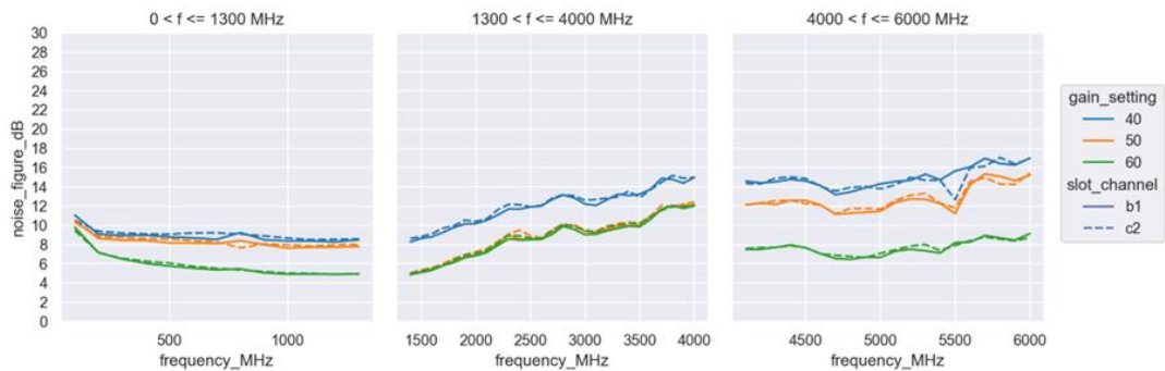
Figure 10.4.10.17: NF as function of frequency. Tree fixed gain settings.
