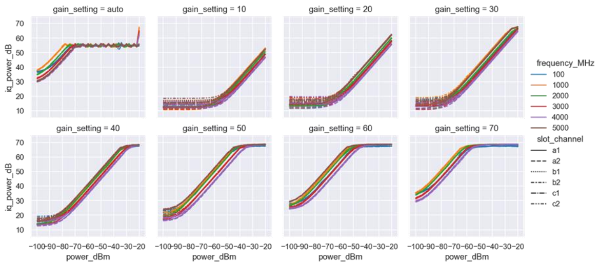
Figure 10.4.10.13. I/Q level vs. input power. Auto gain settings vs. fixed gain setting
