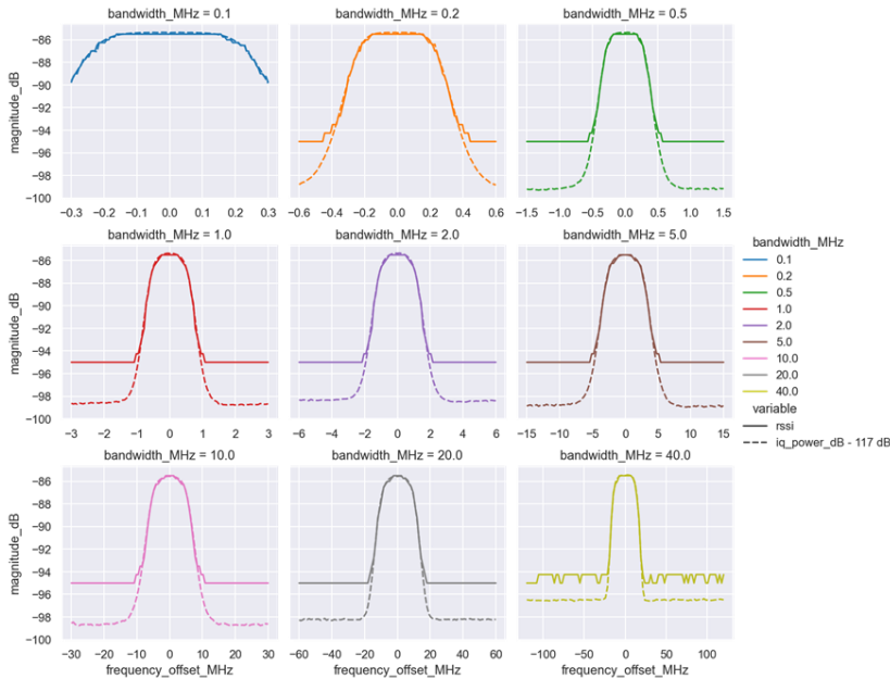
Figure 10.4.10.14. RX BW vs. RX filter setting
