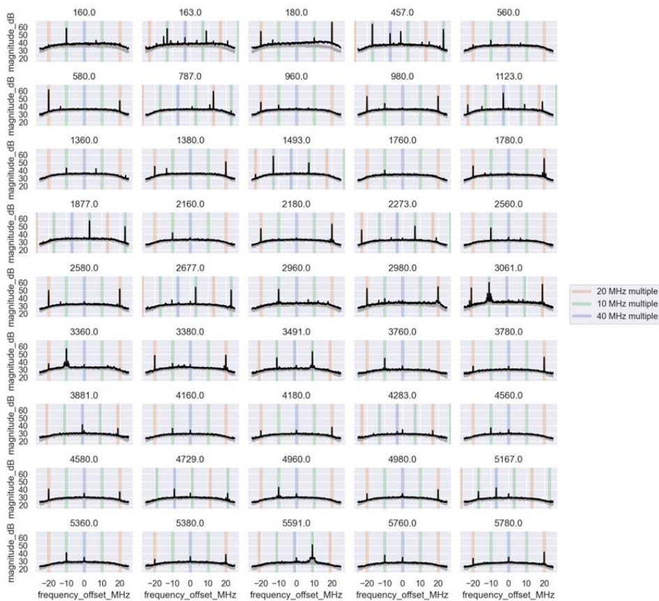
Figure 10.4.10.20. RX internal generated spurious.
