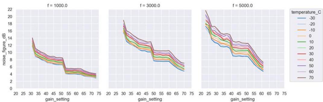
Figure 10.4.10.18. NF as function of temperature
