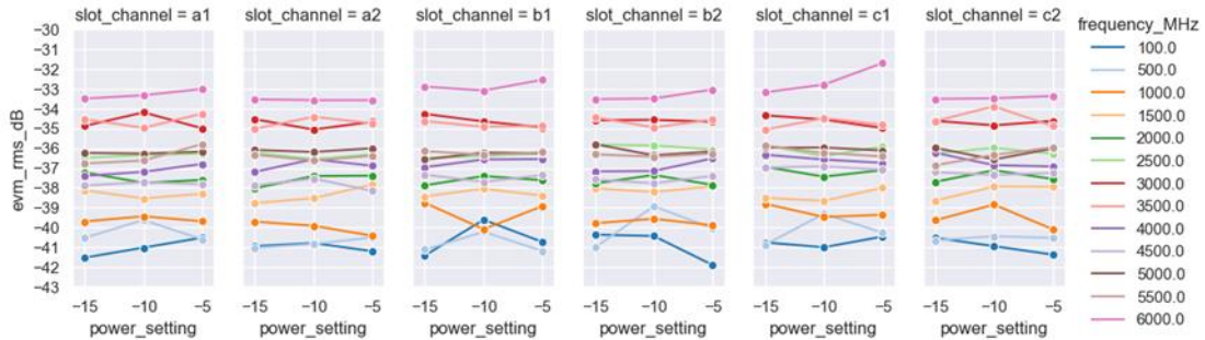
Figure 10.4.10.9. Typical EVM values. TX scale_setting 0.7
