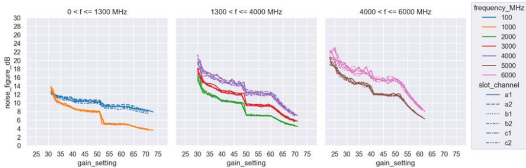
Figure 10.4.10.16. NF as function of RX Gain setting
