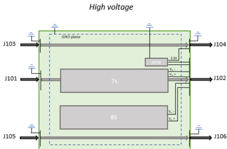
Figure 4-1: Block diagram of Panel
