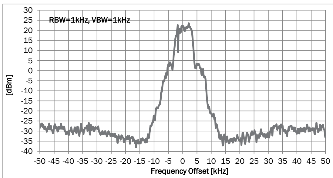
Figure 2 AX100U + UL Narrow Band TX spectrum 4800 baud, GFSK, m=0.667
