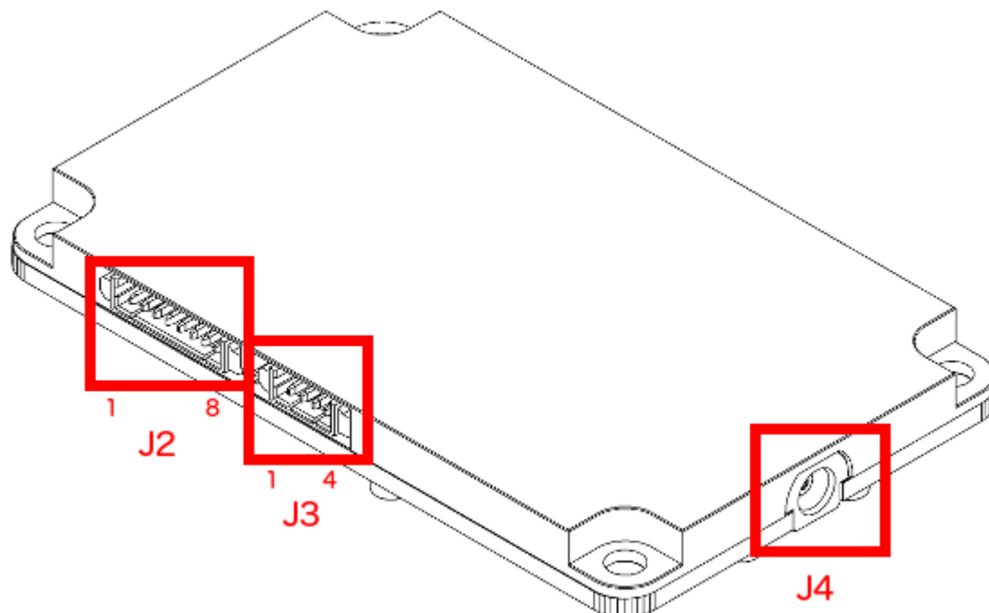
Figure 1 AX100 top connectors
