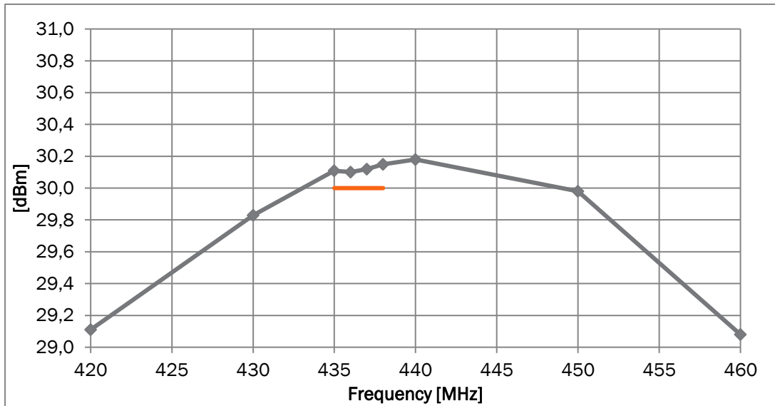
Figure 3 AX100U Output power versus frequency
