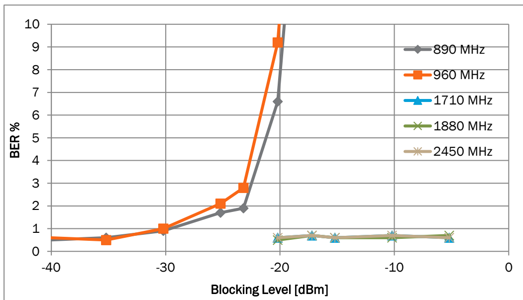
Figure 9 Ground Frequency blocking performance
