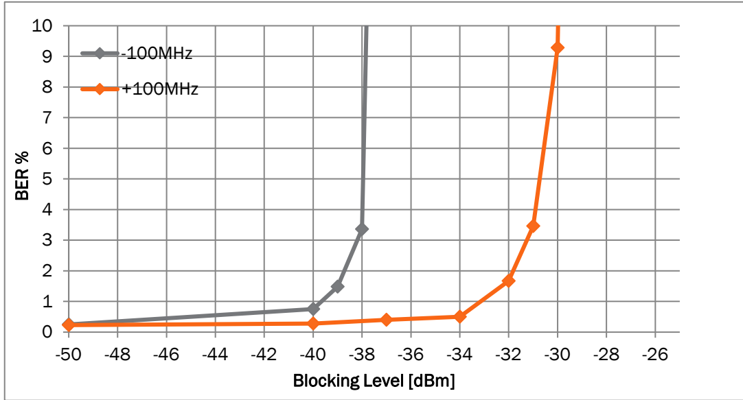
Figure 8 Far blocking performance
