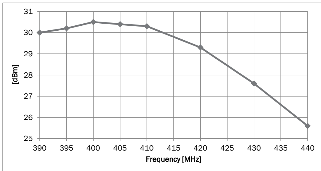
Figure 4 AX100UL Output power versus frequency
