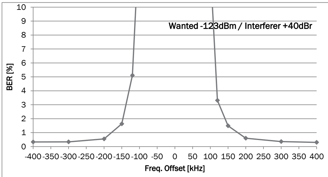
Figure 10 Narrowband blocking at 401 MHz, wanted -123 dBm, interferer +40 dB
