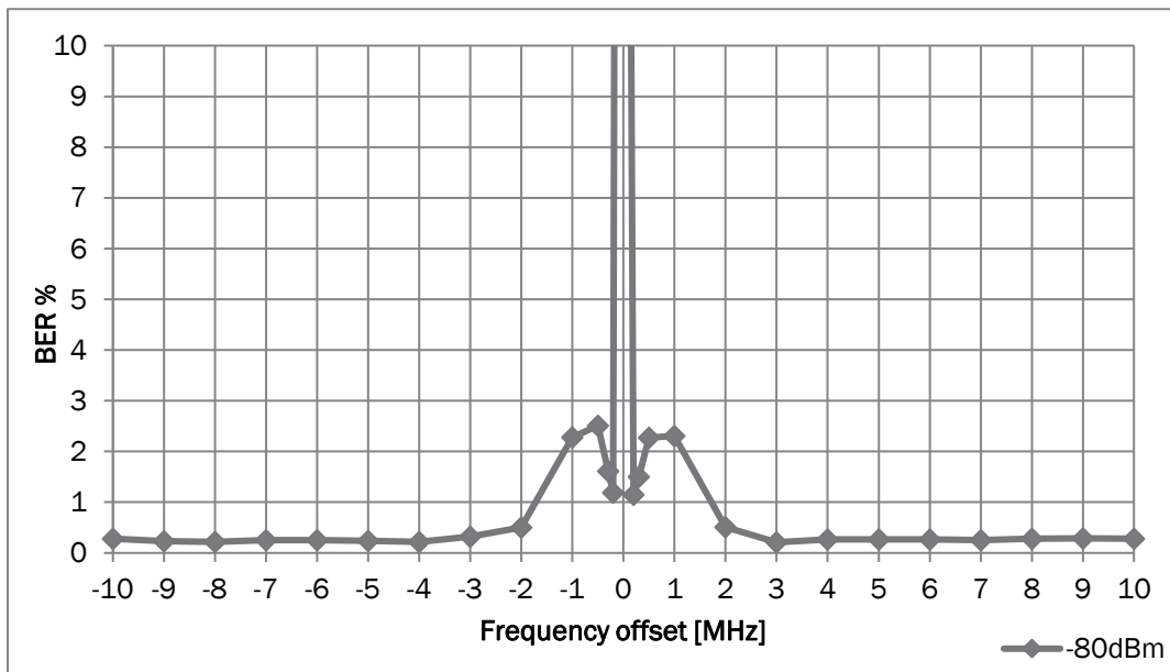
Figure 7 Blocking performance
