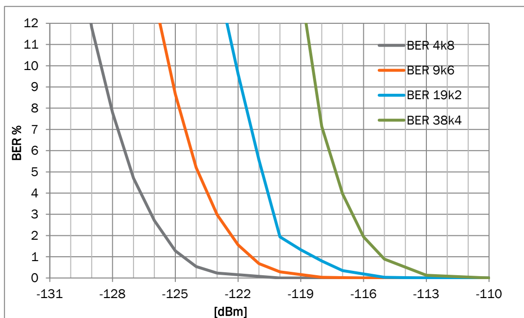
Figure 5 Receiver sensitivity
