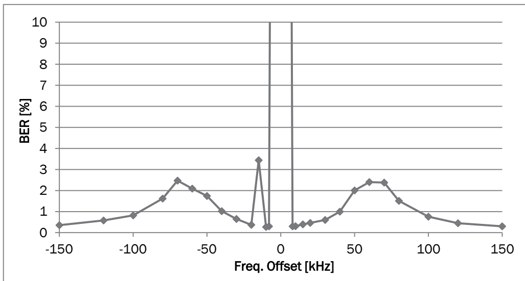
Figure 11 Narrowband blocking at 401 MHz, wanted -123 dBm, interferer +30 dB
