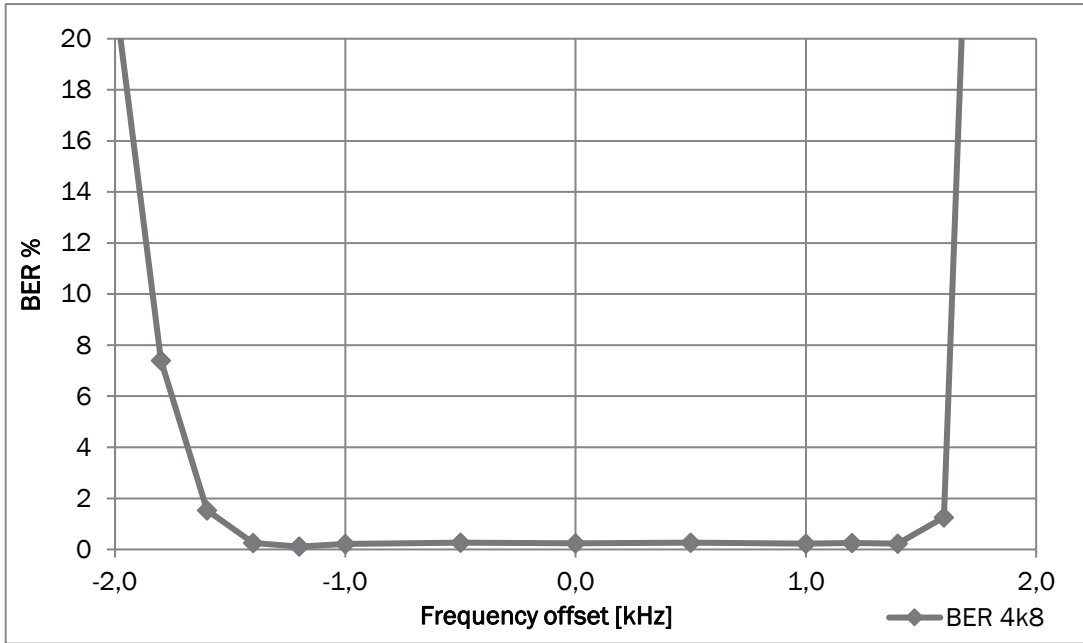
Figure 6 AFC performance
