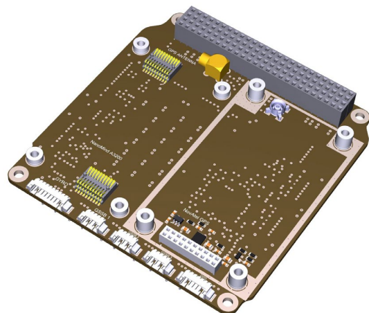
Figure 4 CAD of NanoDock ADCS-6
