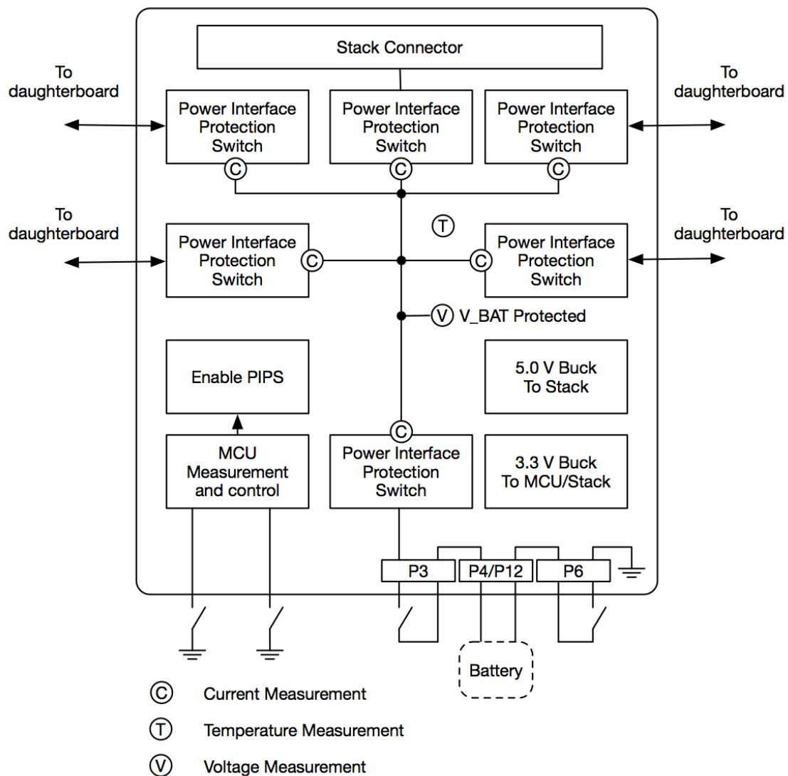
Fig. 2.1: P60 Dock Block Diagram
