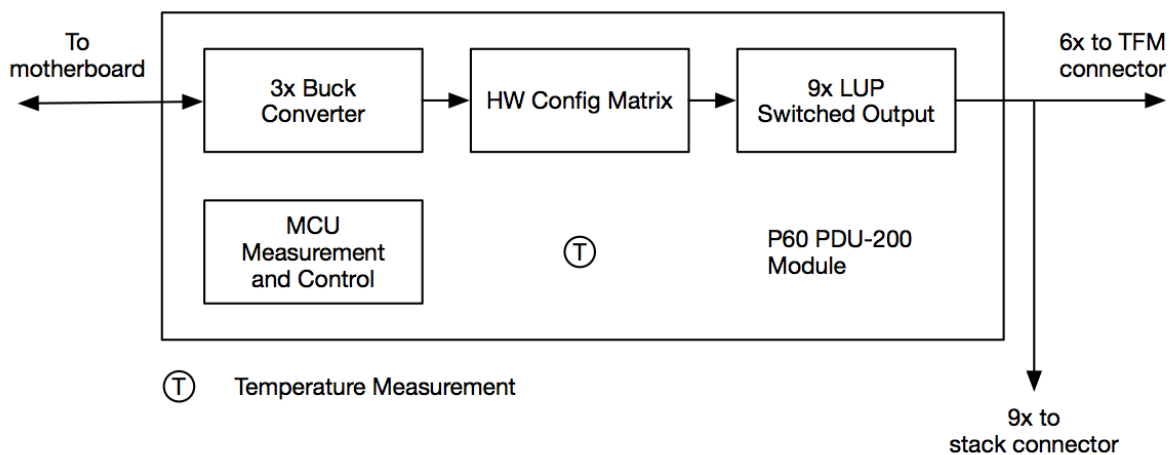
Fig. 2.1: P60 PDU-200 Block Diagram
