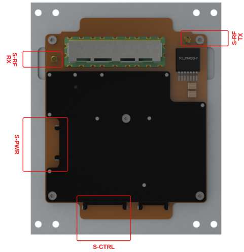
(b) NanoCom ANT2150-DUP bottom view.
