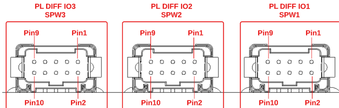
Figure 4.11: SPW1, SPW2 and SPW3 pinout.
