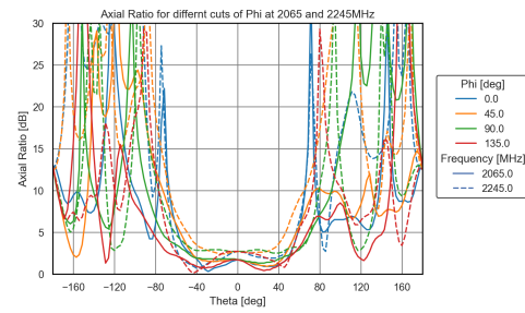
(b) S-Band axial ratio at 2065 MHz to 2245 MHz.
