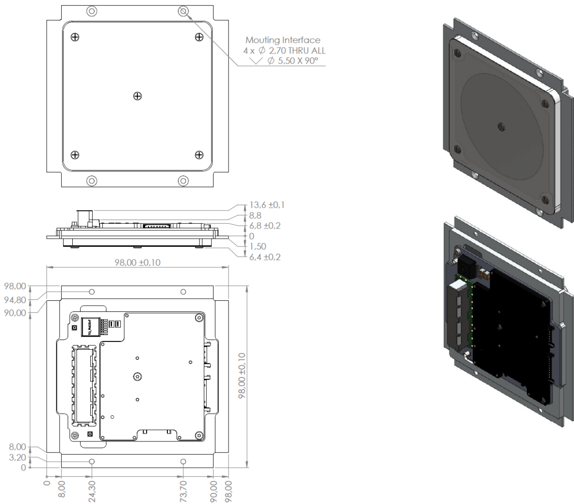
Figure 11.6: ANT2150 Backplate Type C.
