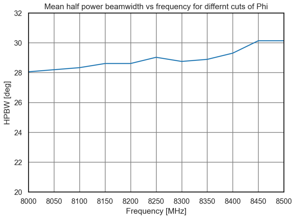
Figure 7.7: X-Band half power beamwidth.
