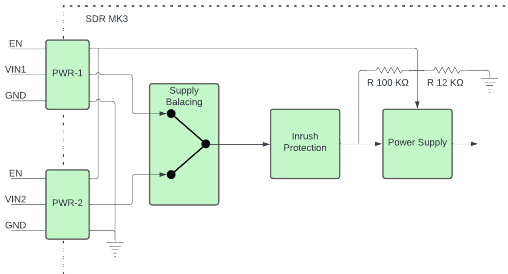
Figure 4.6: SDR MK3 power supply interface.
