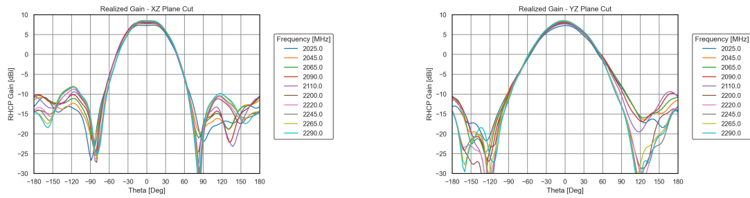
(a) S-Band realized gain vs Theta, XZ plane.
