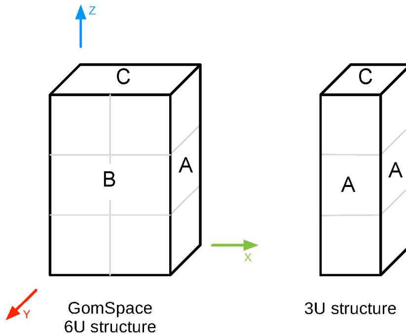
Figure 11.1: Antenna mounting plate Type ABC and XYZ side definitions.
