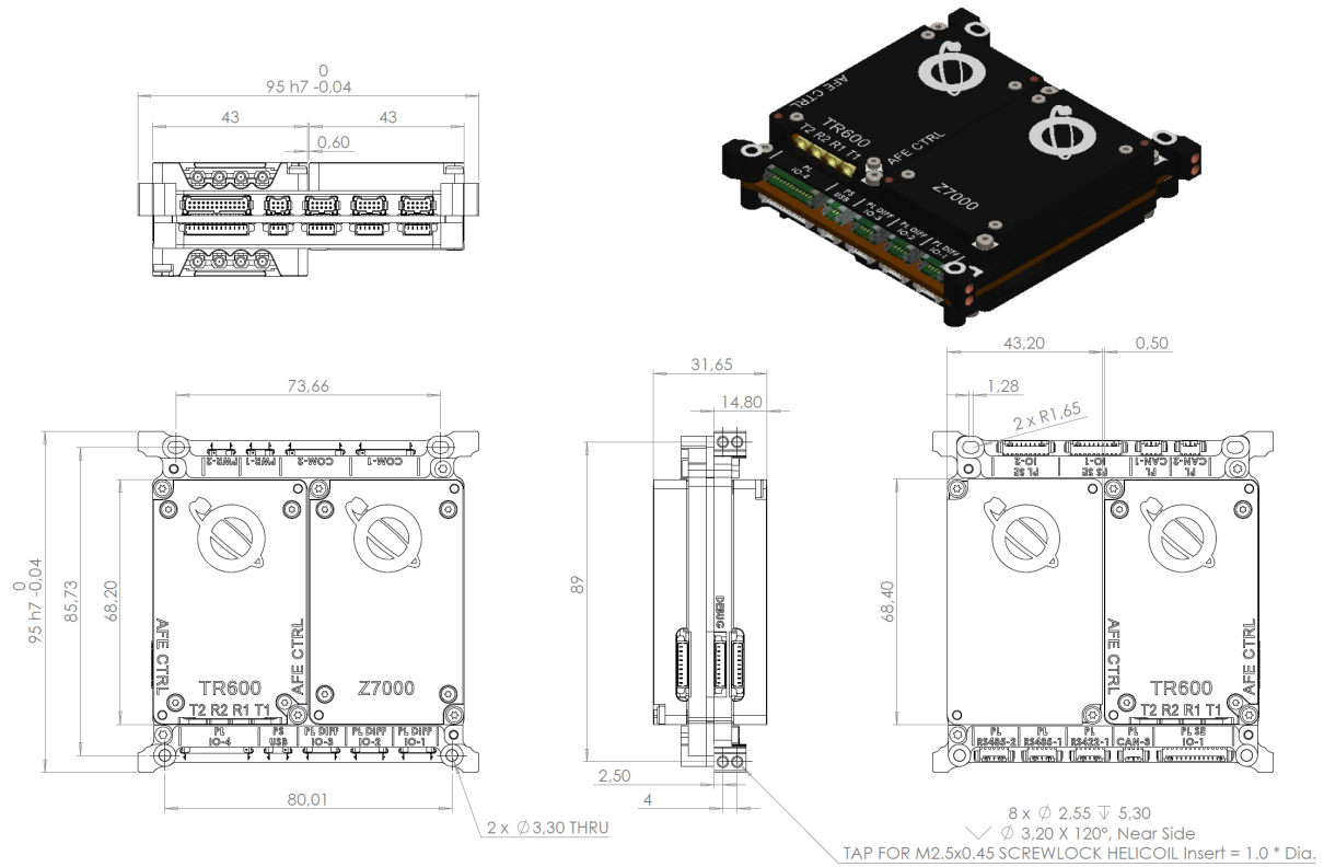
Figure 11.4: SDR MK3 - NanoCom Link SX.
