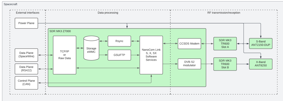
Figure 2.1: High-level system overview.
