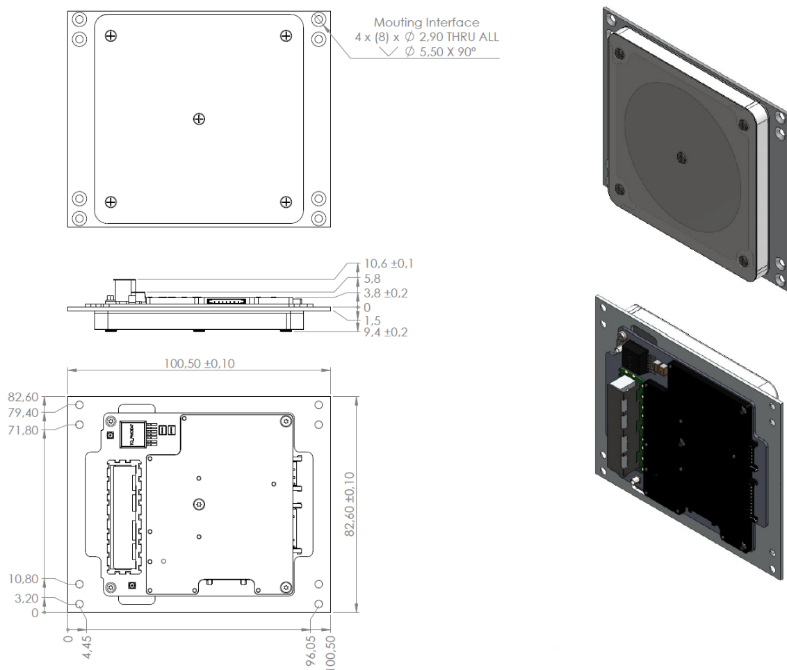
Figure 11.5: ANT2150 Backplate Type A.
