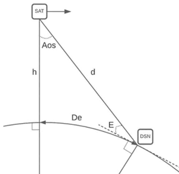
Figure 6.15: Satellite and DSN station geometry.
