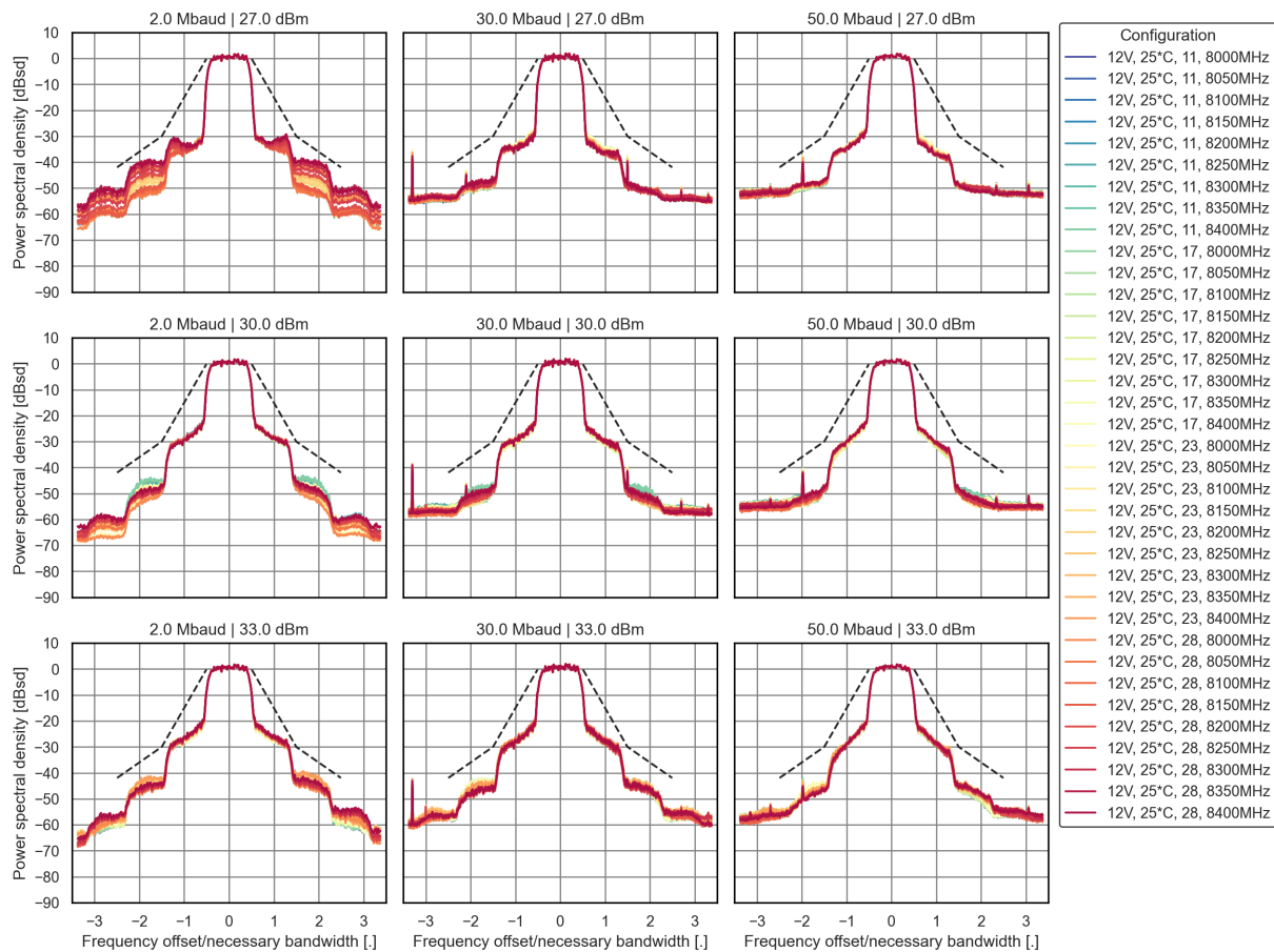
Figure 6.11: Typical spectral emission V_{\text{MAIN-8250}} = 12 \text{ VDC} and T_{\text{AMB}} = +25^\circ \text{C} .
