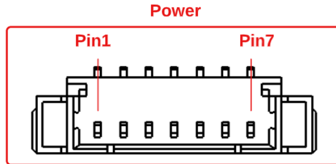
Figure 4.9: ANT8250 X-PWR connector pinout.
