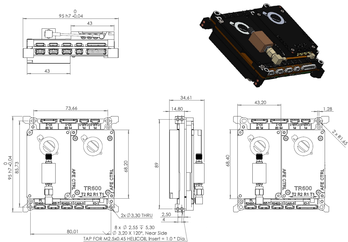
Figure 11.11: IF filter attached to SDR MK3 Slot-C cover shield.
