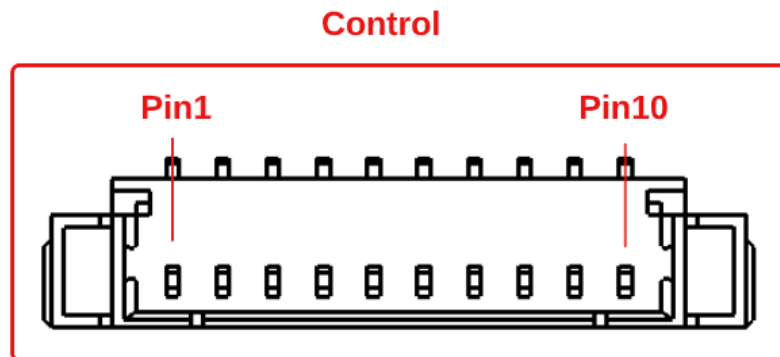
Figure 4.15: ANT8250 X-CTRL connector pinout.
