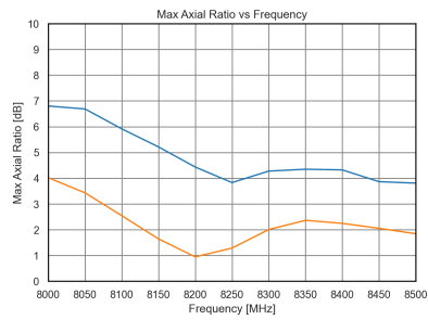
(a) X-Band max axial ratio vs frequency.
