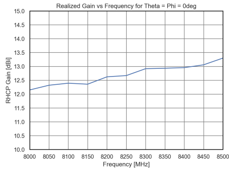
(c) X-Band realized gain for Theta = Phi = 0°.
