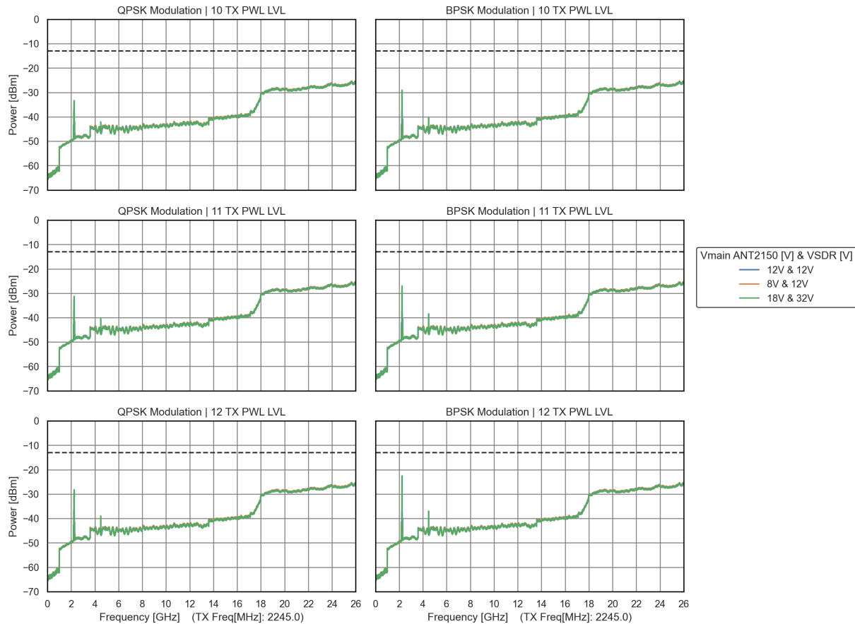
Figure 6.9: Typical spurious emission across extreme conditions.
