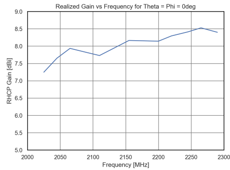
(c) S-Band realized gain for Theta = Phi = 0°.
