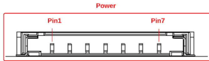
Figure 4.8: ANT2150-DUP S-PWR connector pinout.
