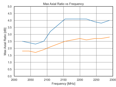
(a) S-Band max axial ratio vs frequency.
