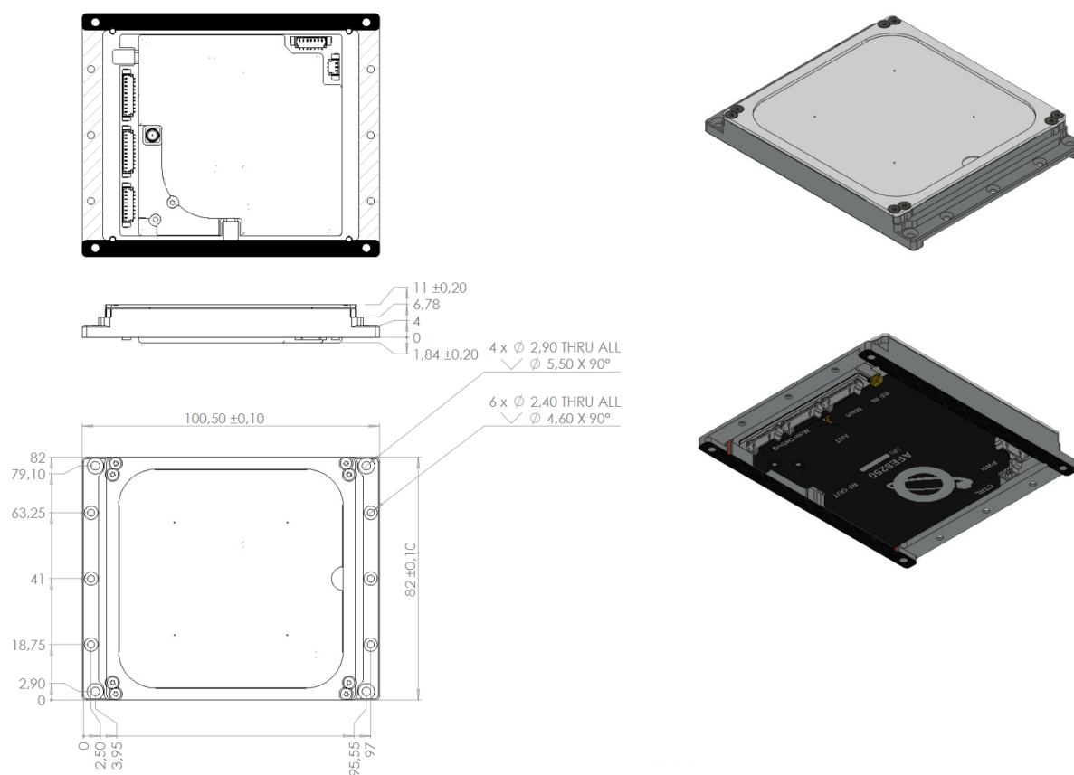
Figure 11.7: ANT8250 Backplate X side.
