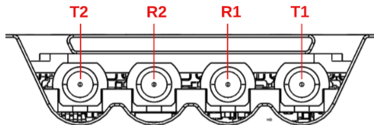
Figure 4.16: TR600 RF connector pinout.
