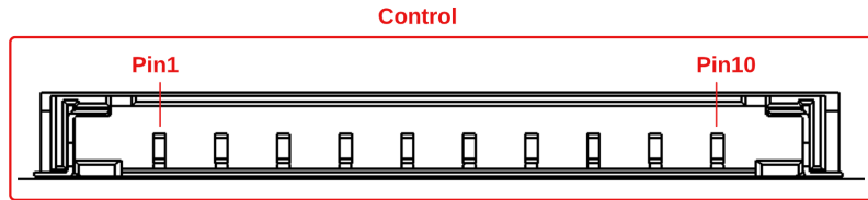
Figure 4.14: ANT2150-DUP S-CTRL connector pinout.
