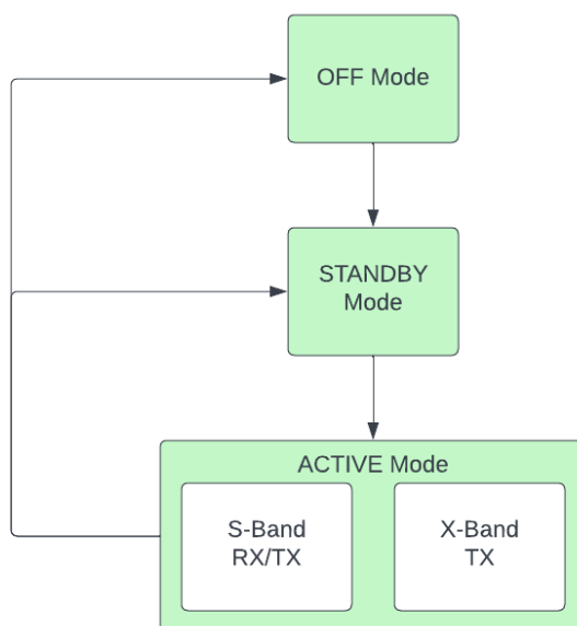
Figure 5.2: Modes of operation.
