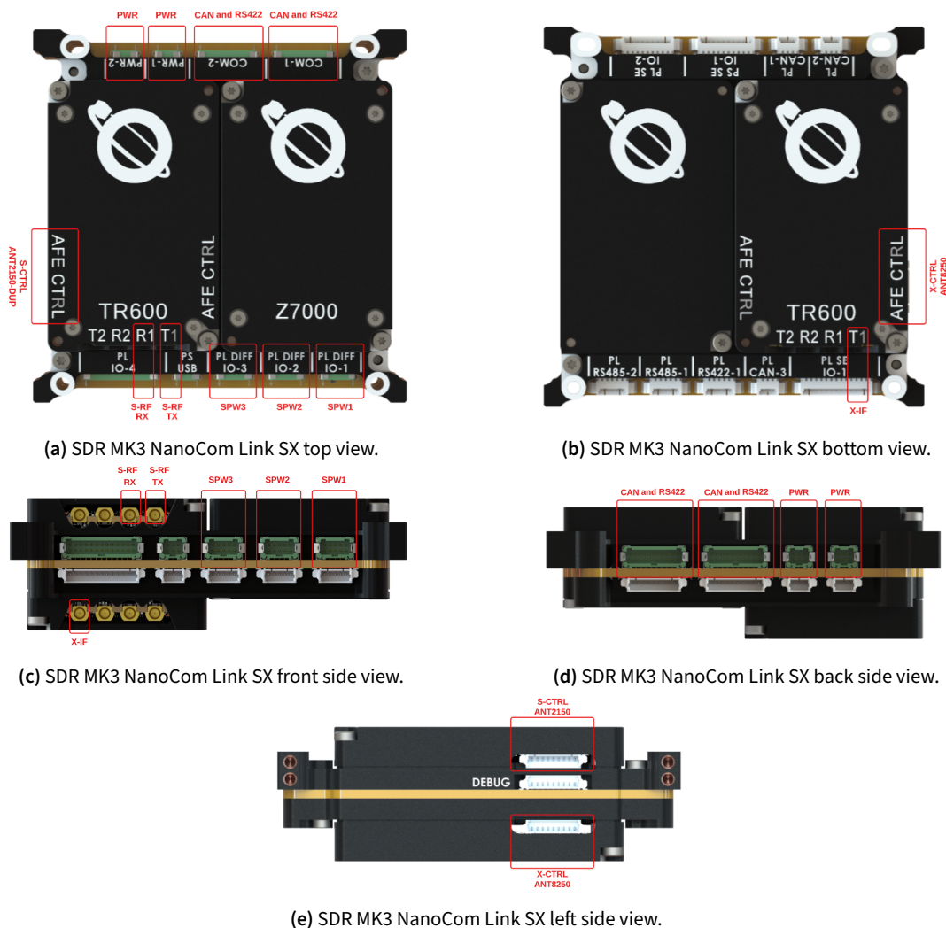
Figure 4.3: Individual connector placements of the NanoCom Link SX variant.
