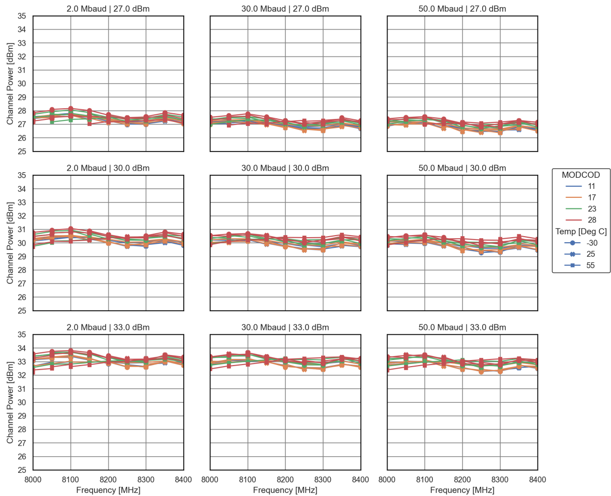
Figure 6.10: Typical channel power vs frequency.
