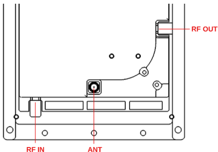
Figure 4.18: ANT8250 RF connector pinout.
