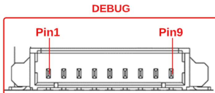
Figure 4.12: DEBUG connector pinout.
