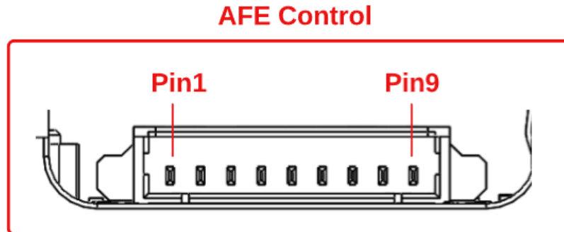
Figure 4.13: TR600 AFE CTRL connector pinout.
