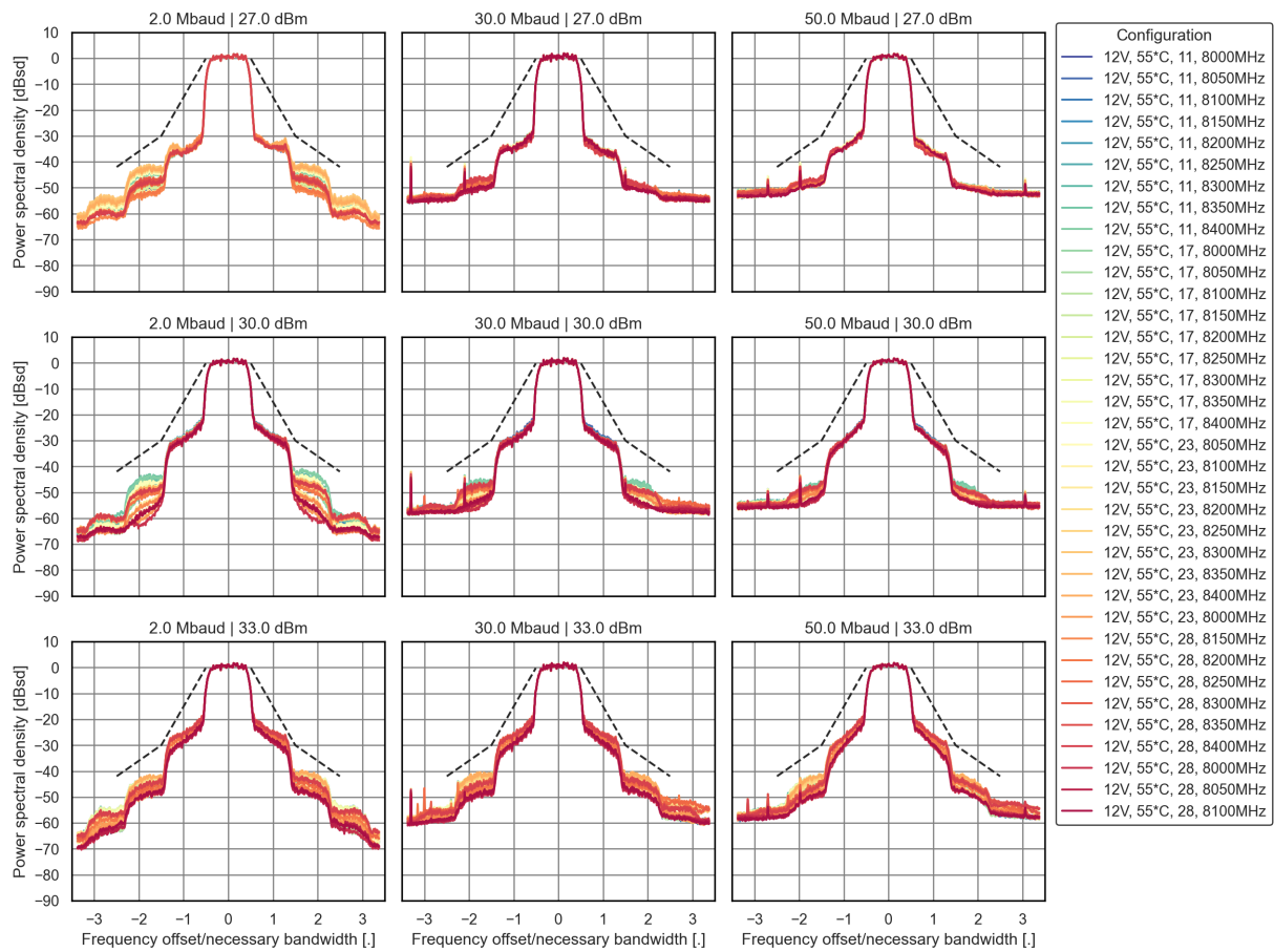
Figure 6.12: Typical spectral emission V_{\text{MAIN-8250}} = 12\text{VDC} and T_{\text{AMB}} = +55^\circ\text{C} .
