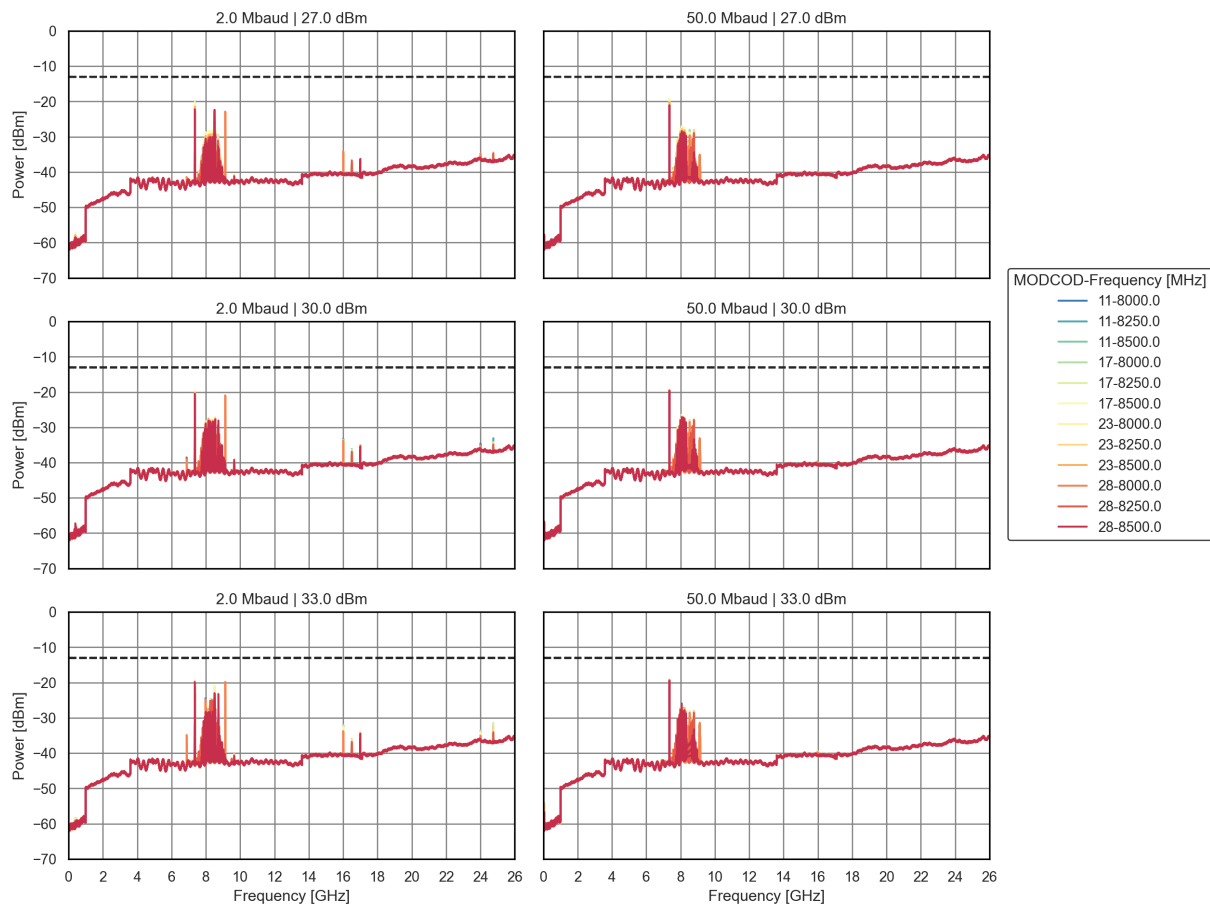
Figure 6.14: Typical spurious emission across extreme conditions.
