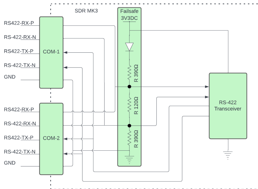
Figure 5.1: RS-422 COM-1 and COM-2 interface.
