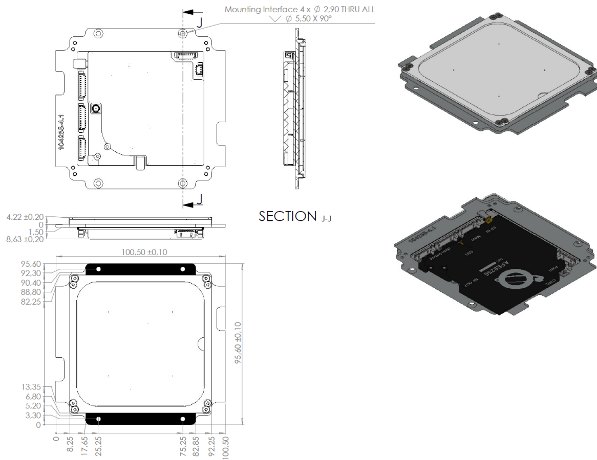
Figure 11.9: ANT8250 Backplate Z side.
