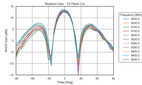
(b) X-Band realized gain vs Theta, YZ plane.
