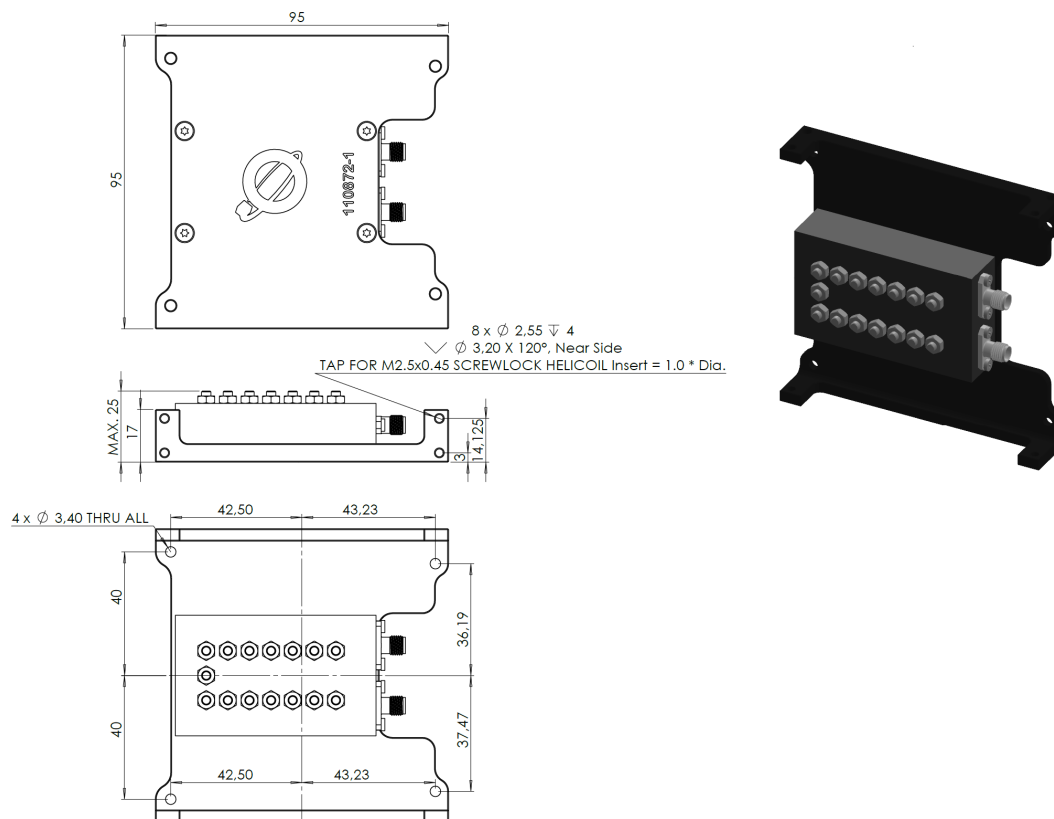
Figure 11.10: RF filter with mounting bracket.
