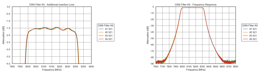
(a) Expected additional loss of the RF filter and coax cables. (b) Frequency response of the RF filter in the DSN Filter Kit.
