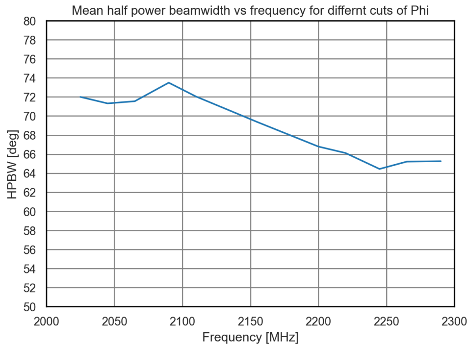
Figure 7.4: S-Band half power beamwidth.
