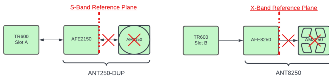
Figure 6.1: Reference plane RF performance characteristics.
