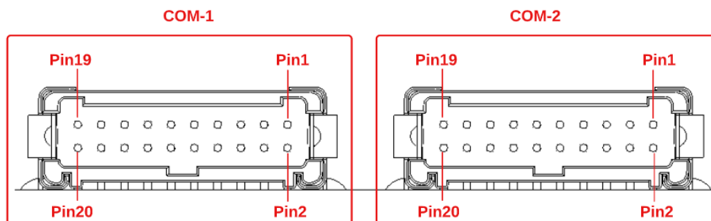
Figure 4.10: COM-1 and COM-2 pinout.
