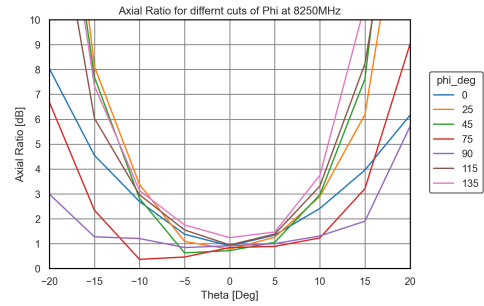
(b) X-Band axial ratio at 8250 MHz.
