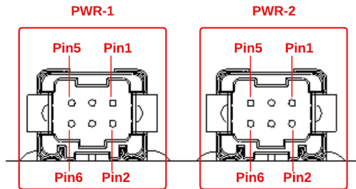
Figure 4.7: PWR-1 and PWR-2 connector pinout.
