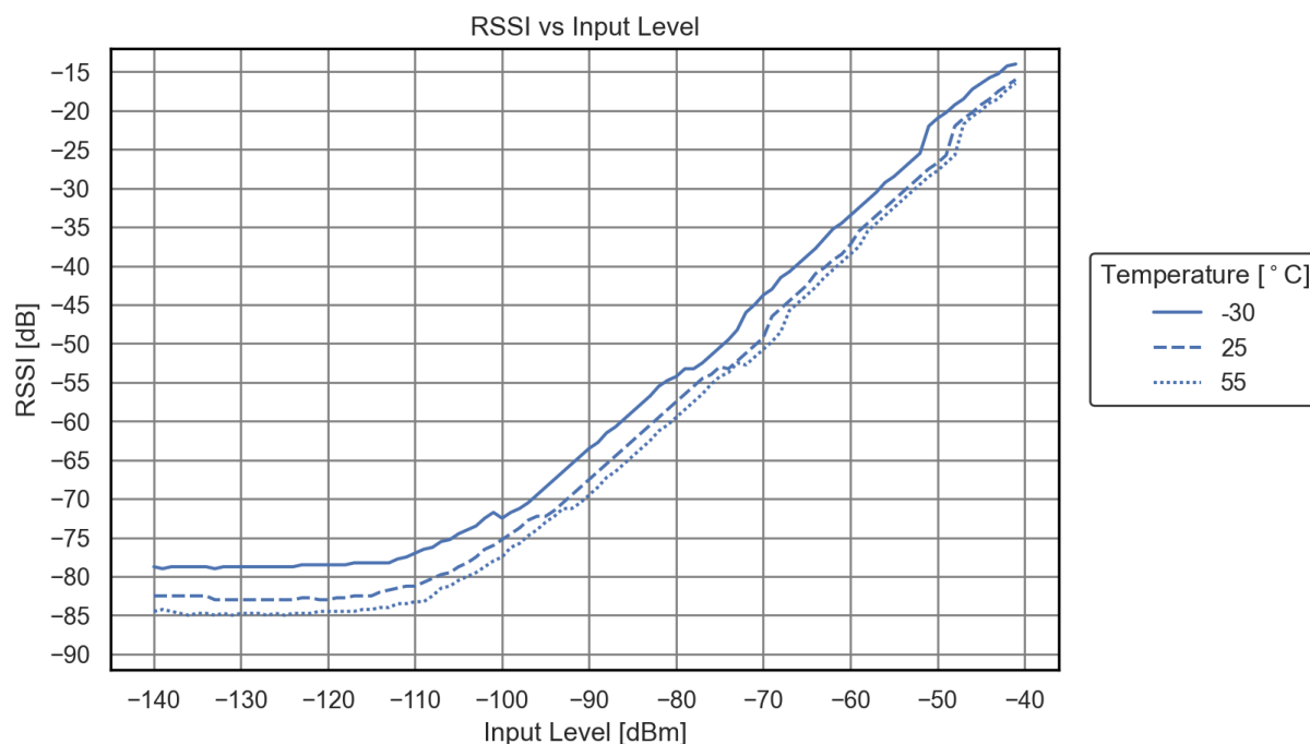
Figure 6.2: Typical RSSI reporting vs RX input level at RX_{FREQ} = 2067 MHz and 2.0 MBd symbol rate.
