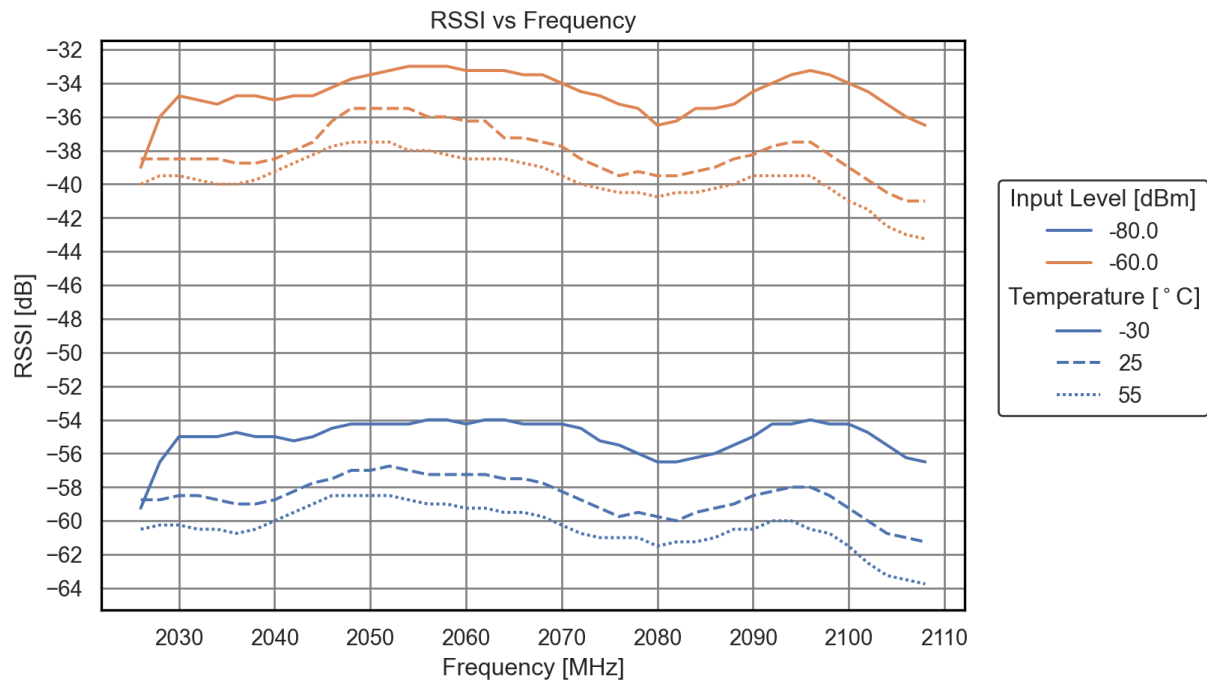
Figure 6.3: Typical RSSI reporting for a fixed RX input level of -60 dBm and -80 dBm.
