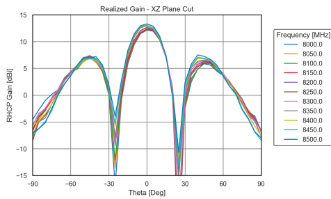
(a) X-Band realized gain vs Theta, XZ plane.
