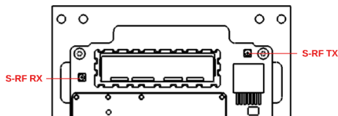
Figure 4.17: ANT2150-DUP RF connector pinout.
