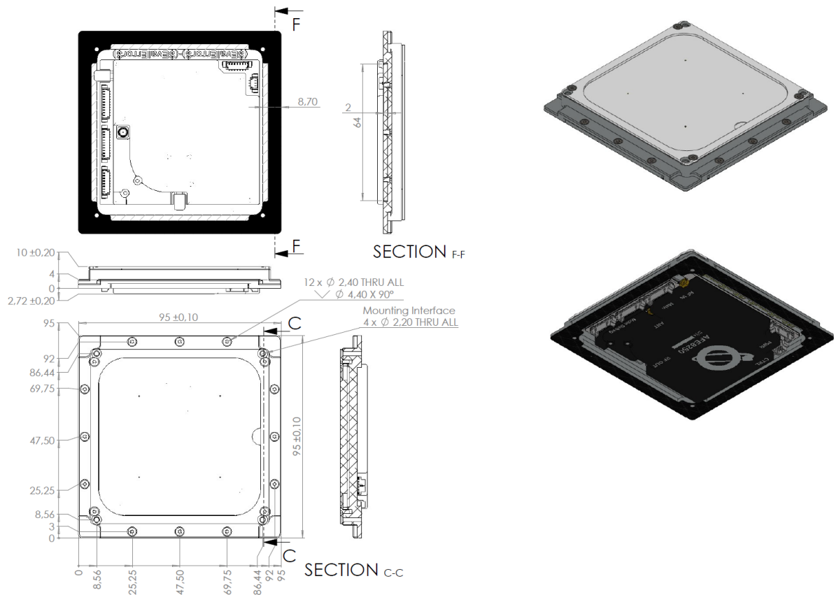
Figure 11.8: ANT8250 Backplate Y side.
