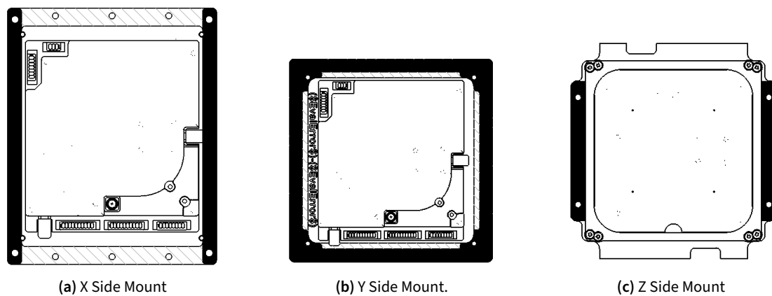
Figure 10.1: ANT8250 Standard Thermal Interface (dark shaded areas).
