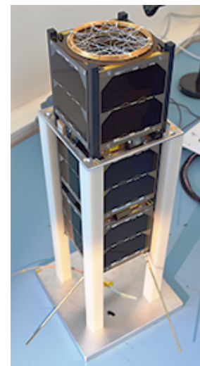
Figure 4 A 3U satellite sitting in an Integration Stand 2
